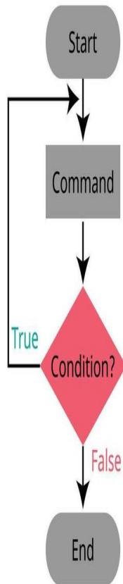
Figure 06:: Loop Flow (For Loop vs While Loop vs Do While Loop)
