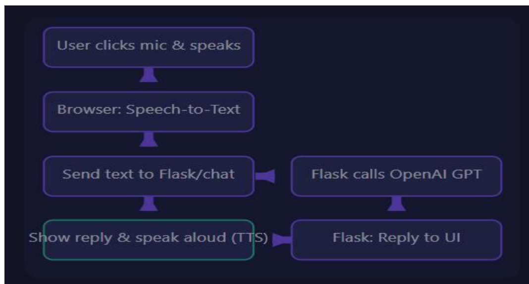
Figure 09 : Workflow of Bolo
